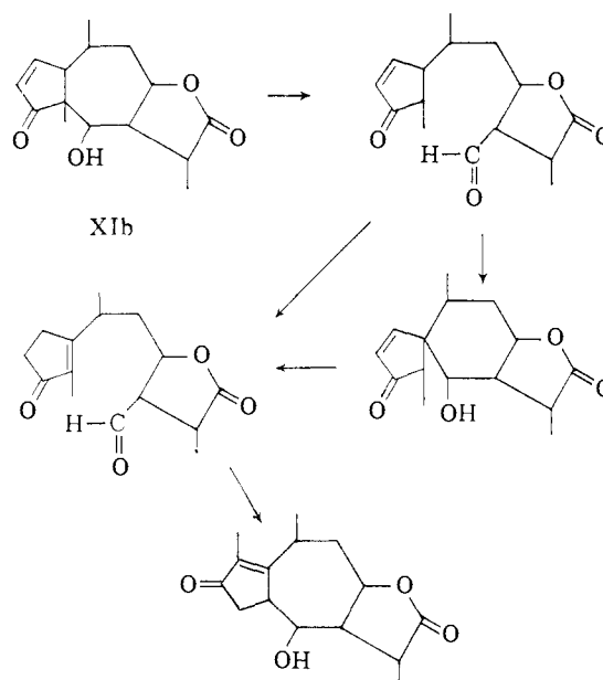
XXXII SCHEME I
